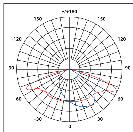
70°x150°
