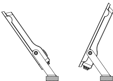
① Pedestal mounting
