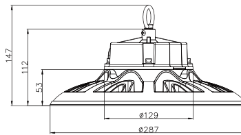
03 ZGSM-HB12-150W □
