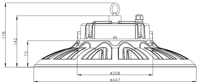
06 ZGSM-HB12-500W □
