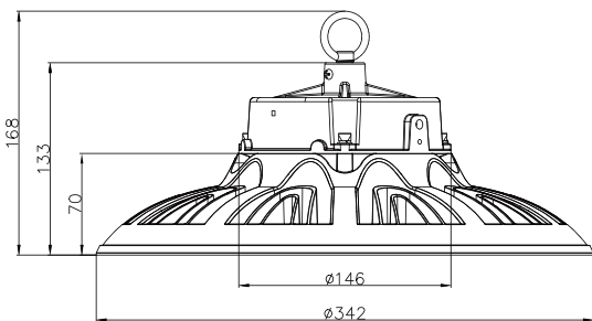
05 ZGSM-HB12-300W □
