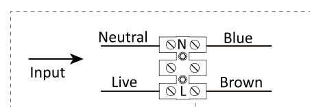
Wiring Diagram 2 - Class II BASED
