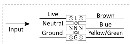
Wiring Diagram 1 - Class I BASED
